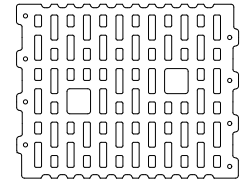
Lochbild 6) T1,4-240
