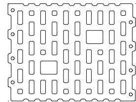
Lochbild 6) T1,4-240
